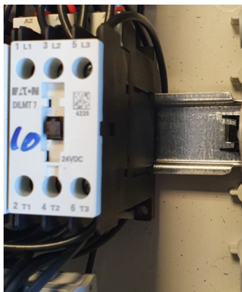
Figuur 4: relais in de rail.
